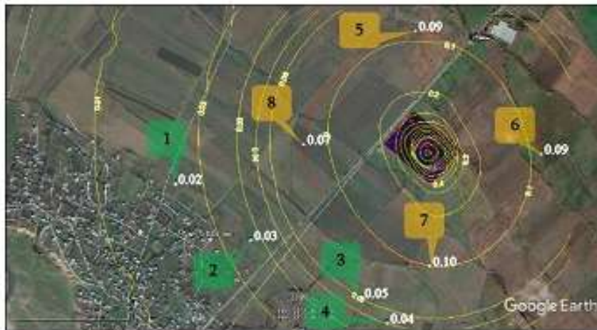
Maximum concentration of total impact group 6046 (codex 337-2908) at control points (nos. 1-4), at the nearest settlements and at the border of 500-m rated zone (nos. 5-8)
