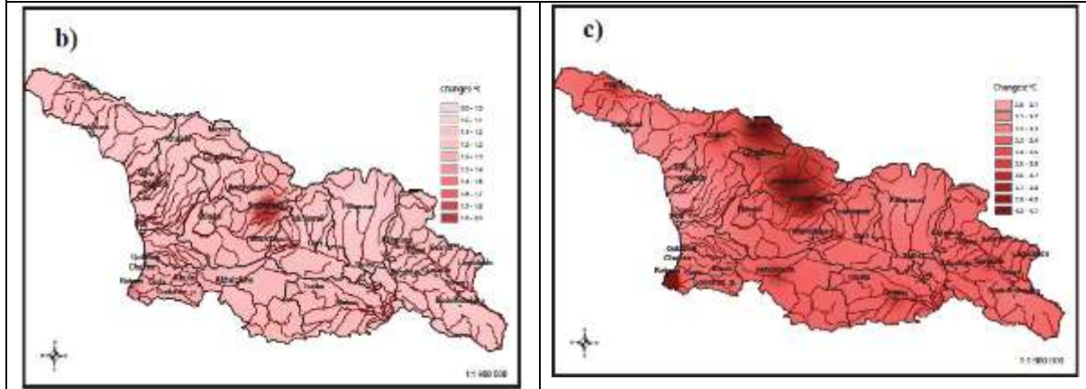
Figure 5.2.2.2: Change of average annual temperature; b) 1986–2010 and 2021–2050; c) 1986–2010 and 2021–2050
