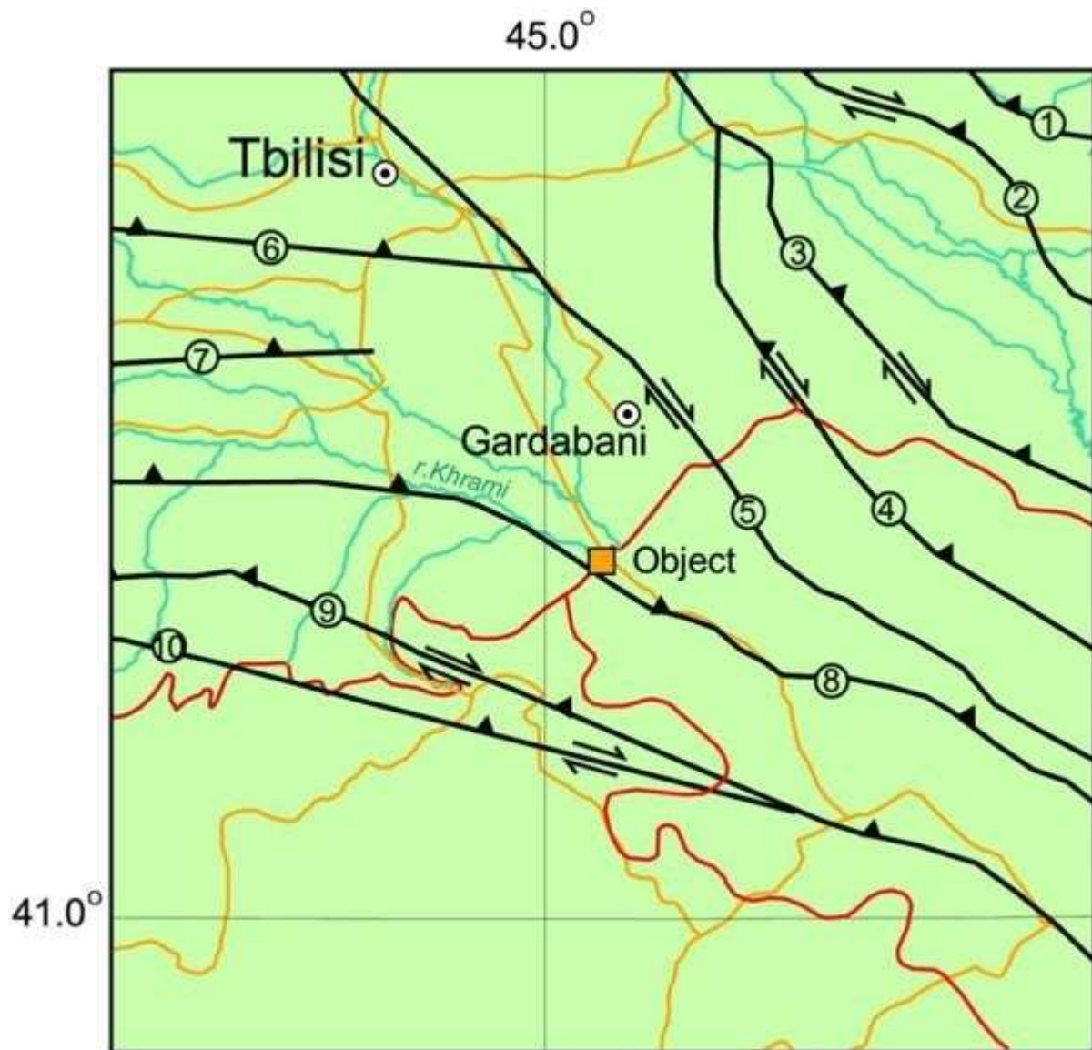
Figure. 5.2.3.4.1.1. Seismically active faults zones (FZ) of the investigation area
