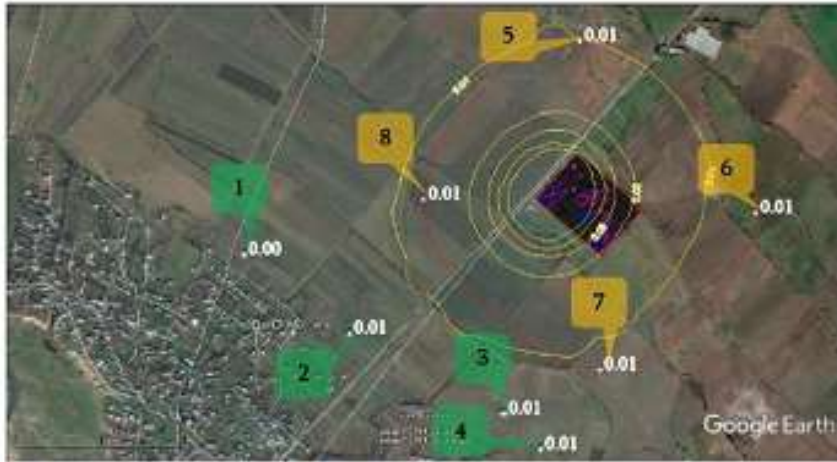
Maximum concentration of incomplete total impact group 6009 (codex 301-330) at control points (nos. 1-4), at the nearest settlements and at the border of 500-m rated zone (nos. 5-8)
