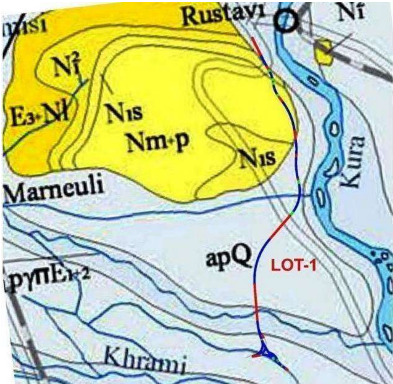
Figure 5.2.3.1.1. Geological map of the project area
