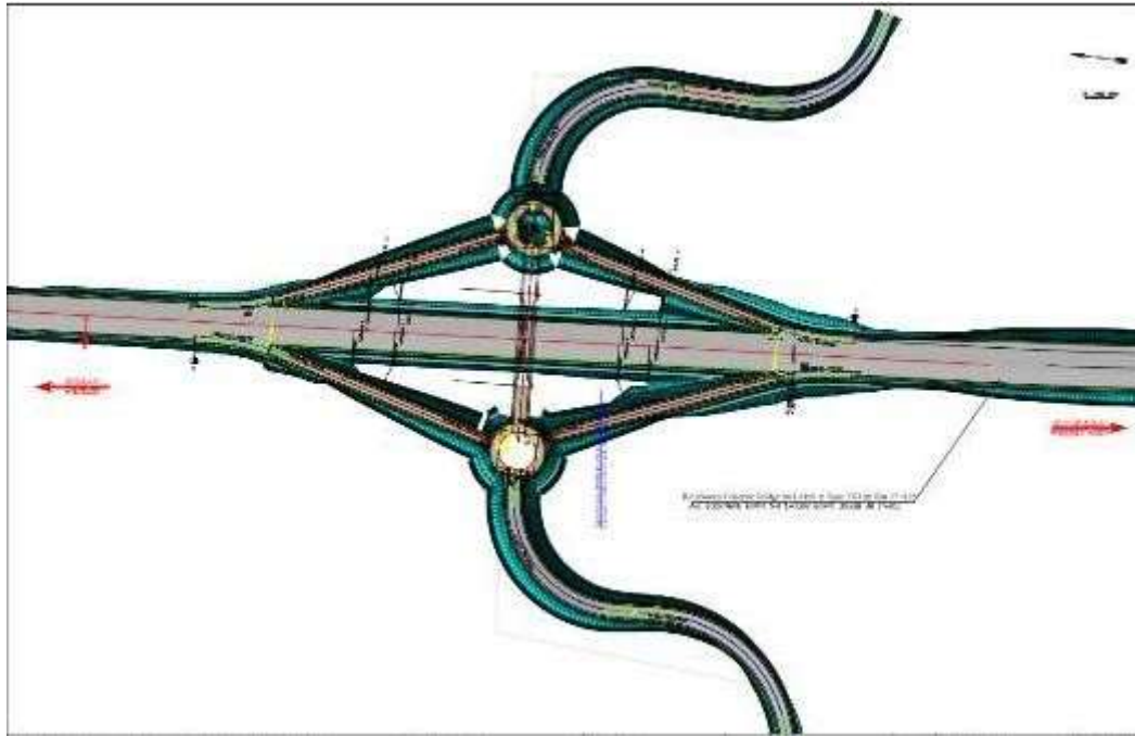
Figure 4.4.3. Azizkendi Interchange 17+305
